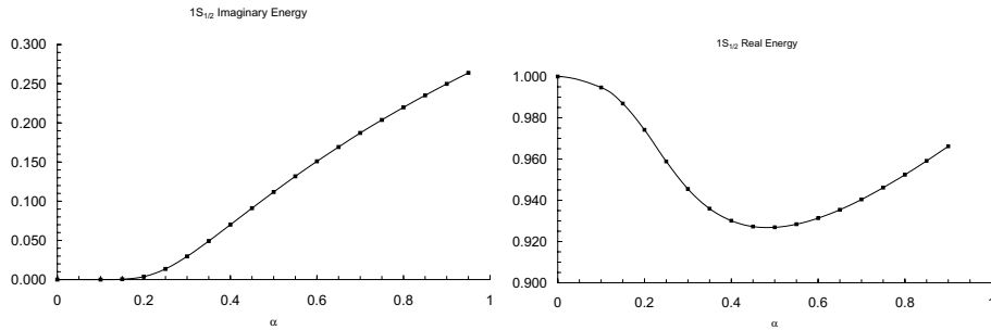
Figure 8: The imaginary and real energies for the 1S_{1/2} state. The left hand plot shows (minus) the imaginary component of the energy as a function of the coupling strength. As expected, this increases as the orbits become more tightly bound. For comparison, the more complicated behaviour of the real part of the energy is shown on the right-hand side.
