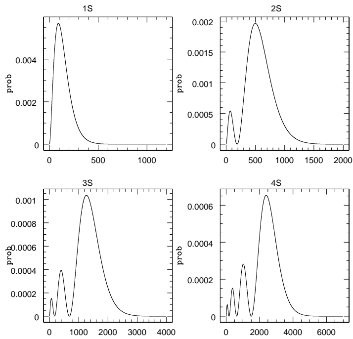
Figure 3: The radial probability density for the 1S_{1/2} , 2S_{1/2} , 3S_{1/2} and 4S_{1/2} states for a coupling of \alpha = 0.1 . The horizontal axis is the dimensionless radius x , and the horizon lies at x = 2 . All plots are started from the horizon. The part of the density inside the horizon is not plotted, though in all cases this smoothly approaches the origin.
