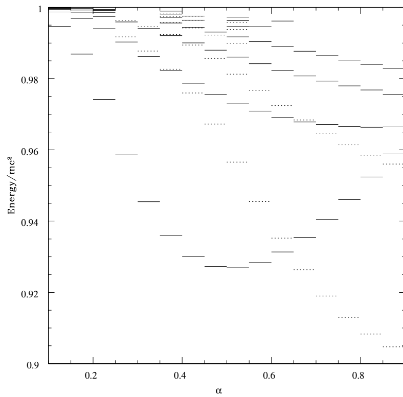
Figure 2: The energy spectra of the S_{1/2} (solid) and P_{1/2} (dashed) states. Beyond a coupling of around \alpha = 0.65 the 2P_{3/2} state takes over as the system's ground state.
