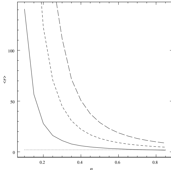
Figure 6: The expectation value of r , in units of GM/c^2 , for the 1S_{1/2} , 2S_{1/2} and 3S_{1/2} states. These are the solid, short dashed and long dashed lines respectively. The broken horizontal line is the horizon.
