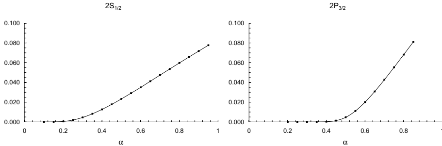
Figure 9: The imaginary energies for the 2S_{1/2} (left) and 2P_{3/2} (right) states. These increase monotonically with the coupling strength, but are considerably lower than the equivalent 1S_{1/2} values.
